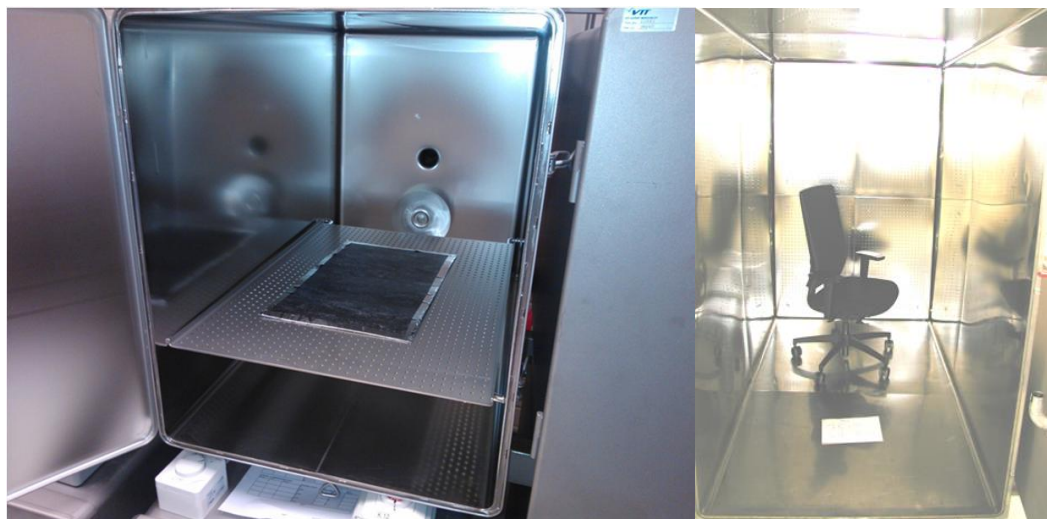
Picture 7 Emission measurement samples in chambers
